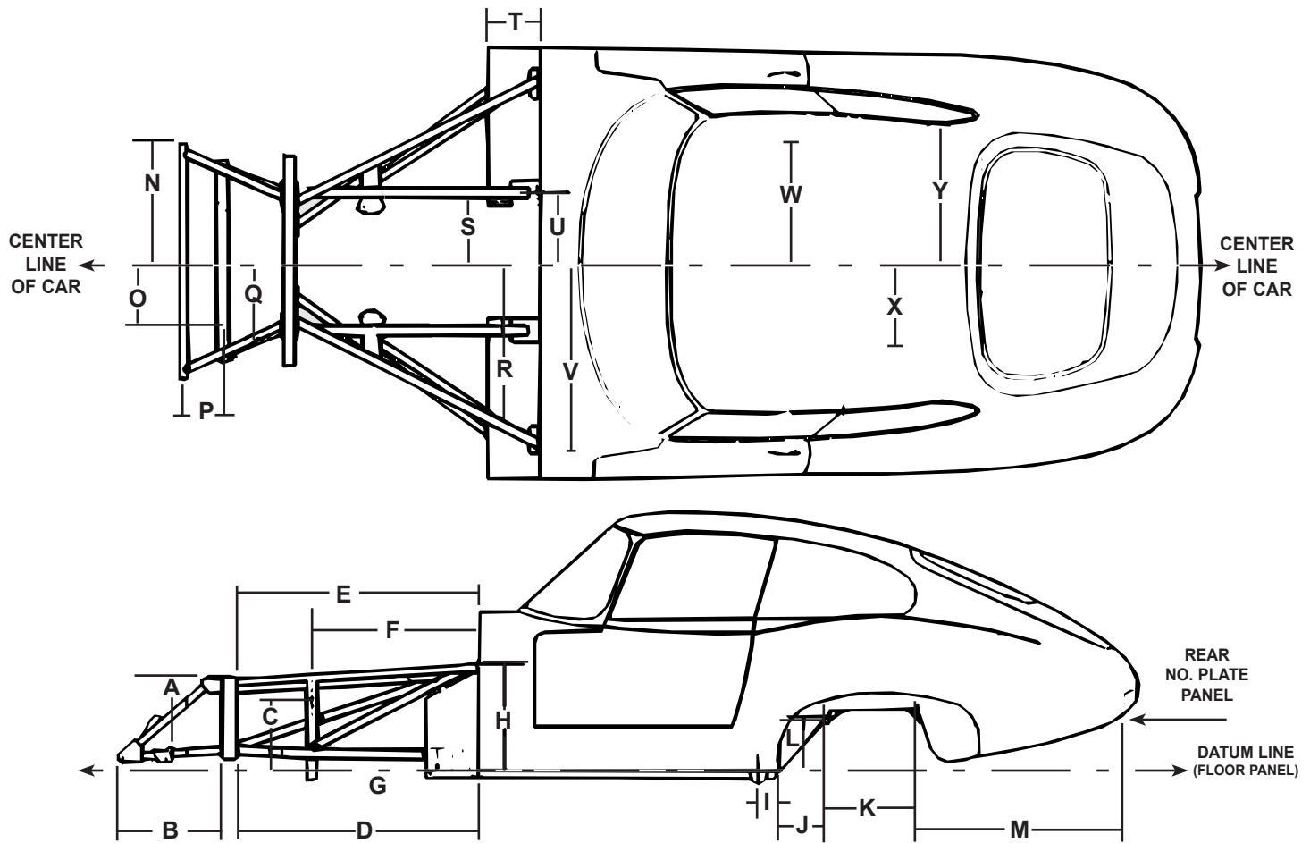
Checking Points for Accidental Damage on XKE Body and Front Frame Section
